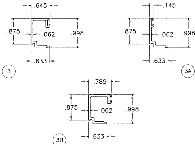
3 3A 3B GLAZING BEADS
